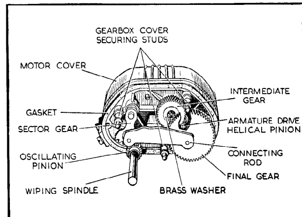
Fig. 2(b) Gearbox incorporating an oscillating pinion and sector gear
