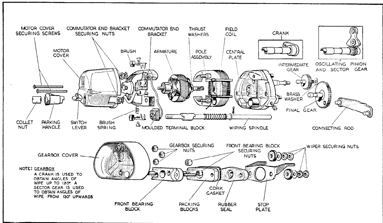
Fig. 3 Dismantled view of wiper
