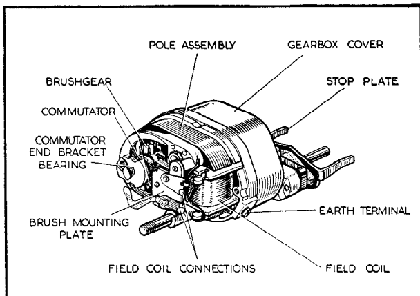
Fig. 1 Wiper with motor cover removed
