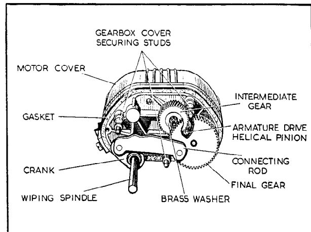
Fig. 2(a) Gearbox incorporating a crank
