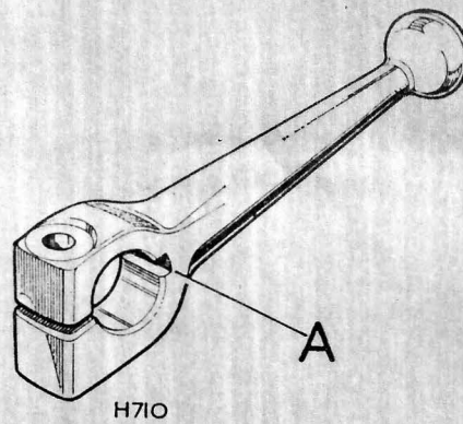
Fig. 1 Modification to gearchange selector levers A—Slot \frac{1}{8} in. (1.5m.m.) x \frac{5}{32} in. (4,0 m.m.)
